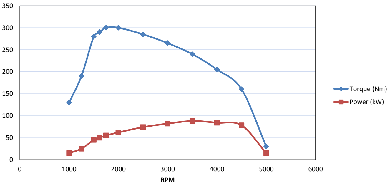
1.5 Duratorq - 120PS (88KW)
